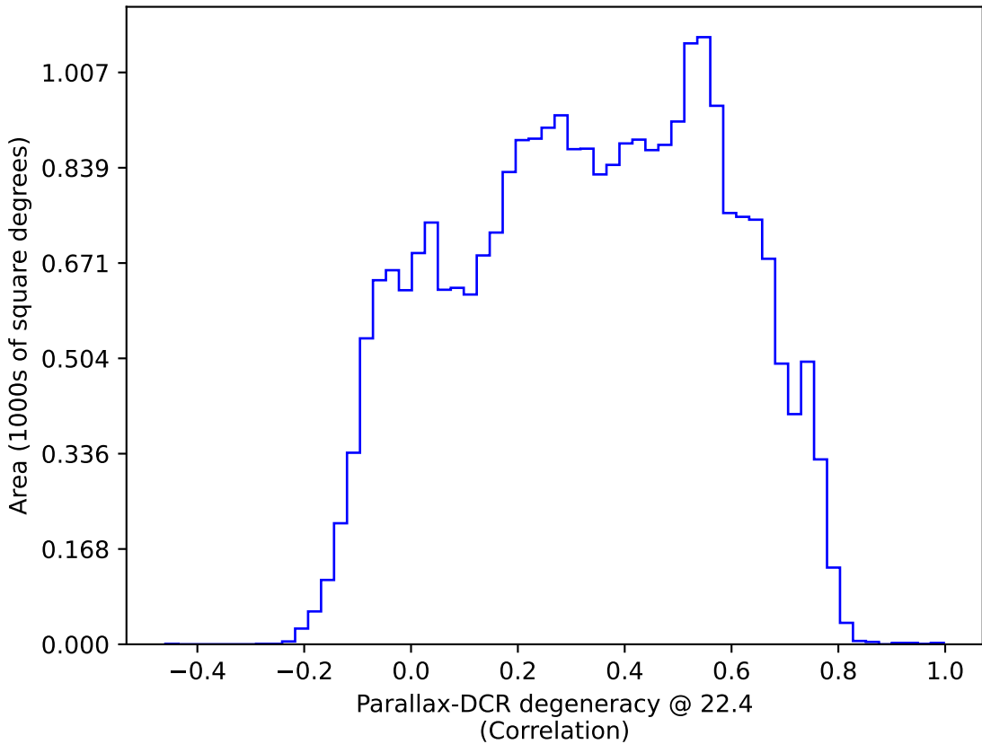
too_100_4v3.4_10yrs : Parallax-DCR degeneracy @ 22.4
