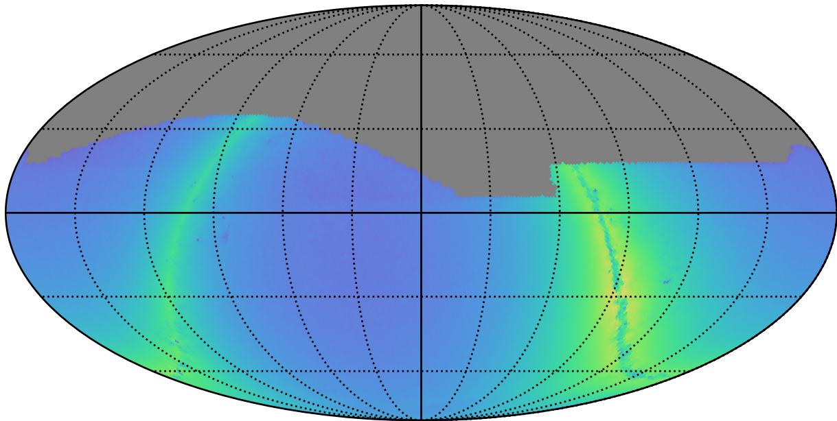
too_100_4v3.4_10yrs z: Nstars_no_crowding
