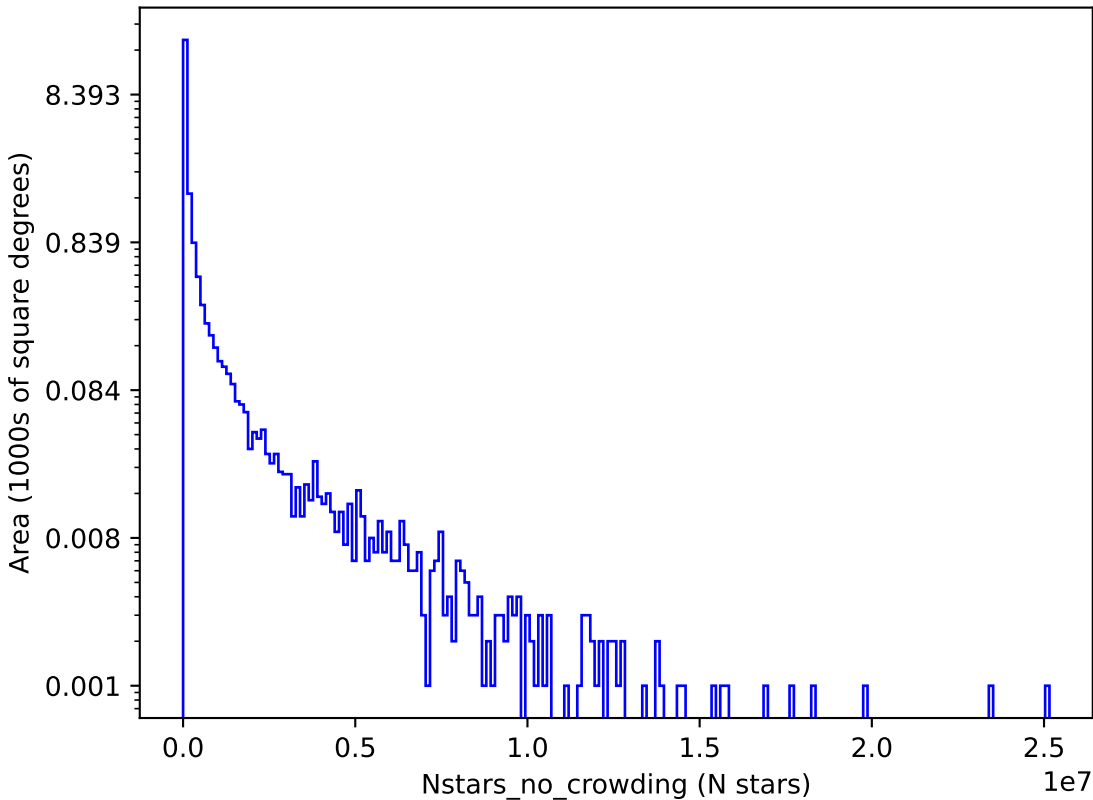
too_100_4v3.4_10yrs y: Nstars_no_crowding
