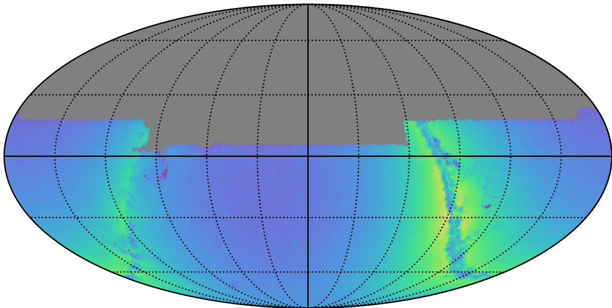
too_100_4v3.4_10yrs u: Nstars_no_crowding
