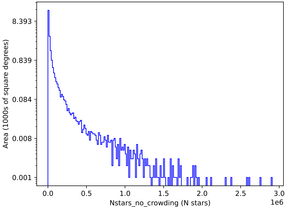
too_100_4v3.4_10yrs u: Nstars_no_crowding
