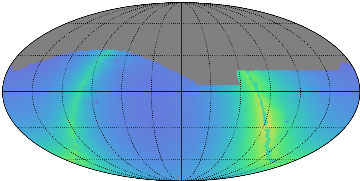
too_100_4v3.4_10yrs r: Nstars_no_crowding
