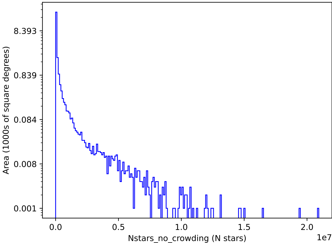
too_100_4v3.4_10yrs r: Nstars_no_crowding
