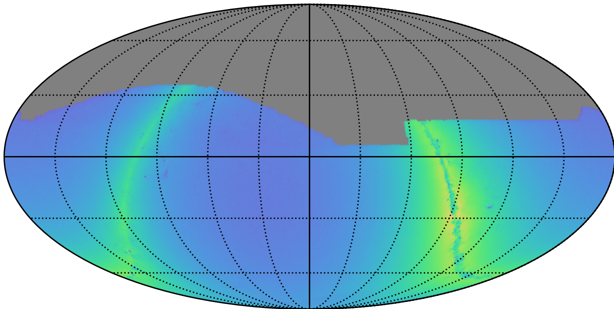
too_100_4v3.4_10yrs i: Nstars_no_crowding
