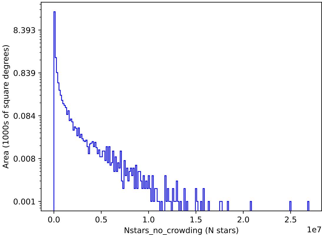
too_100_4v3.4_10yrs i: Nstars_no_crowding
