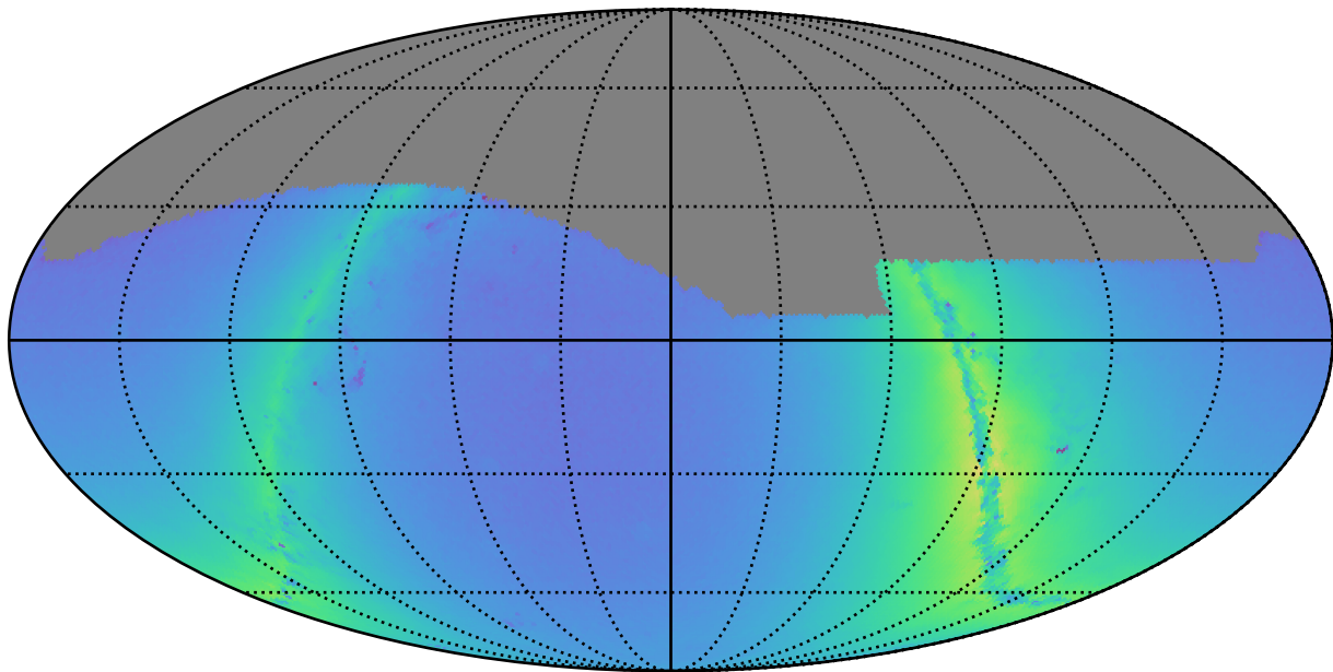
too_100_4v3.4_10yrs g: Nstars_no_crowding
