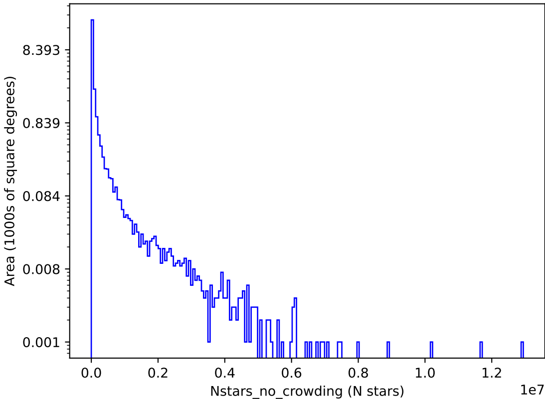
too_100_4v3.4_10yrs g: Nstars_no_crowding
