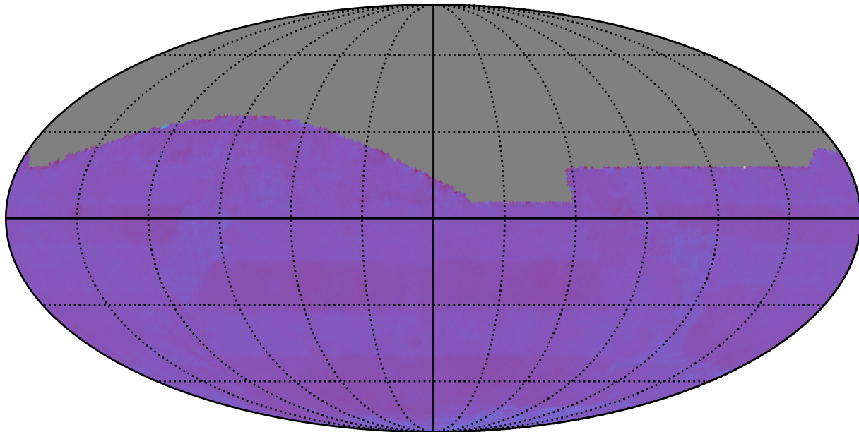
too_100_4v3.4_10yrs : Normalized Proper Motion Uncert @ 24.0
