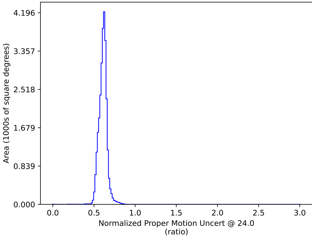
too_100_4v3.4_10yrs : Normalized Proper Motion Uncert @ 24.0
