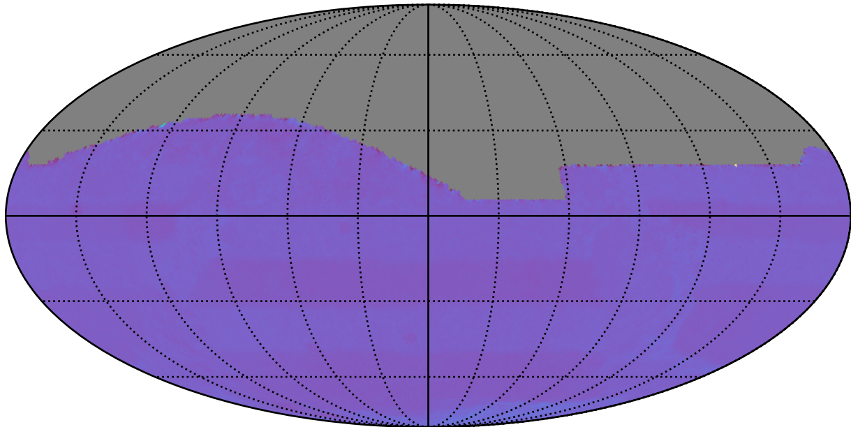
too_100_4v3.4_10yrs : Normalized Proper Motion Uncert @ 20.5
