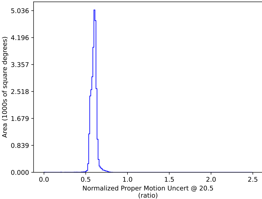
too_100_4v3.4_10yrs : Normalized Proper Motion Uncert @ 20.5
