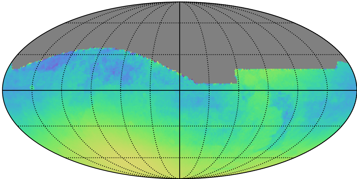
too_100_4v3.4_10yrs : Normalized Parallax Uncert @ 24.0
