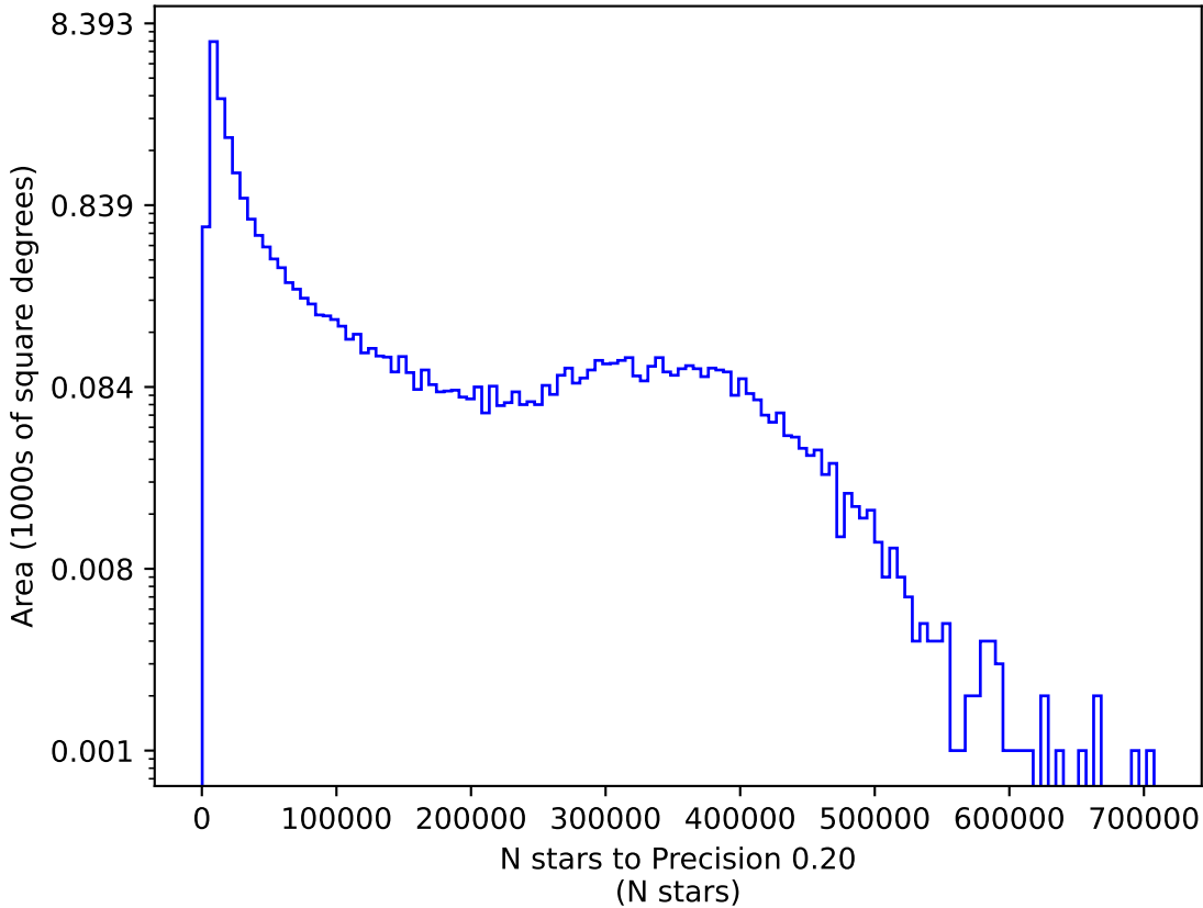
too_100_4v3.4_10yrs y: N stars to Precision 0.20
