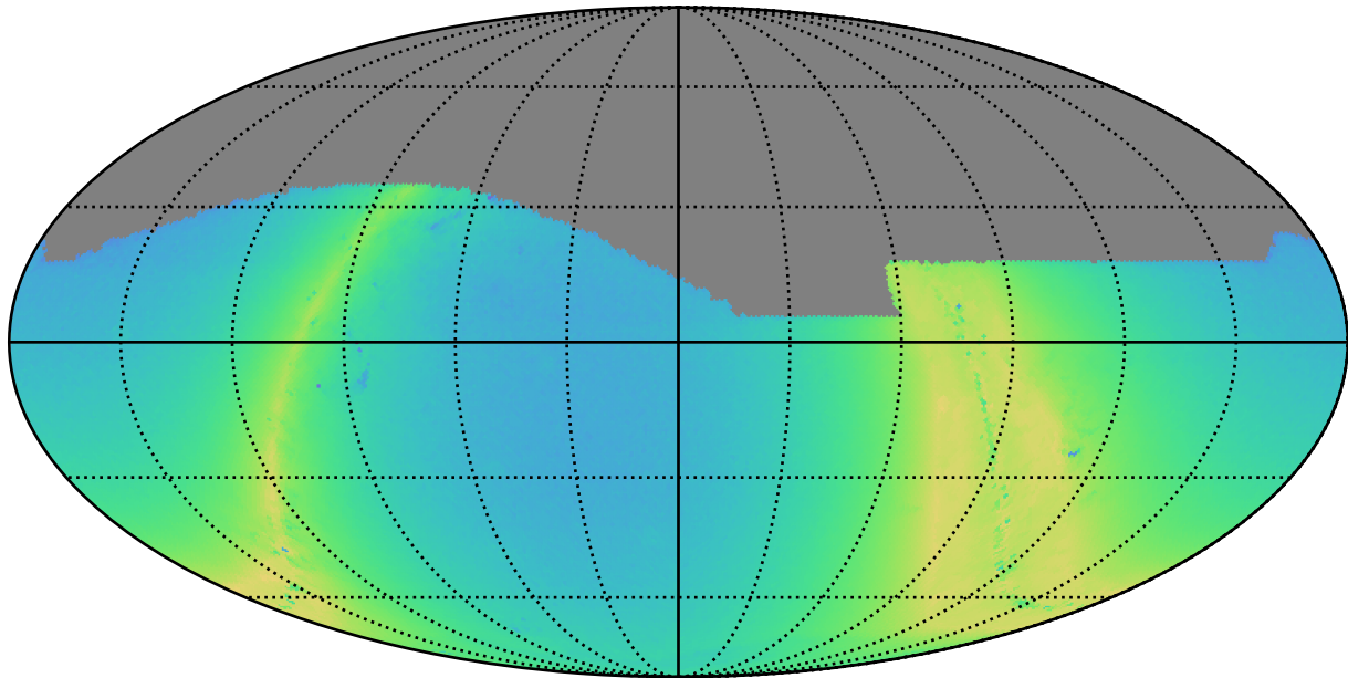
too_100_4v3.4_10yrs r: N stars to Precision 0.20
