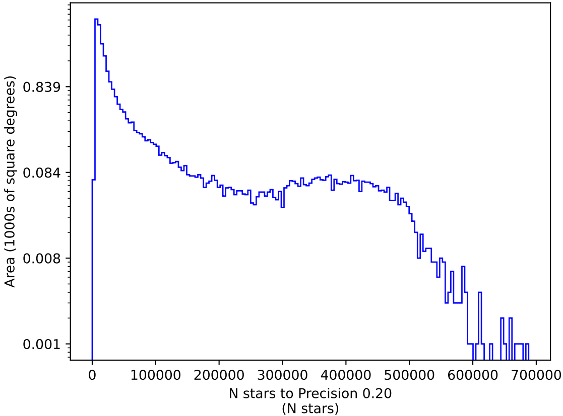
too_100_4v3.4_10yrs r: N stars to Precision 0.20
