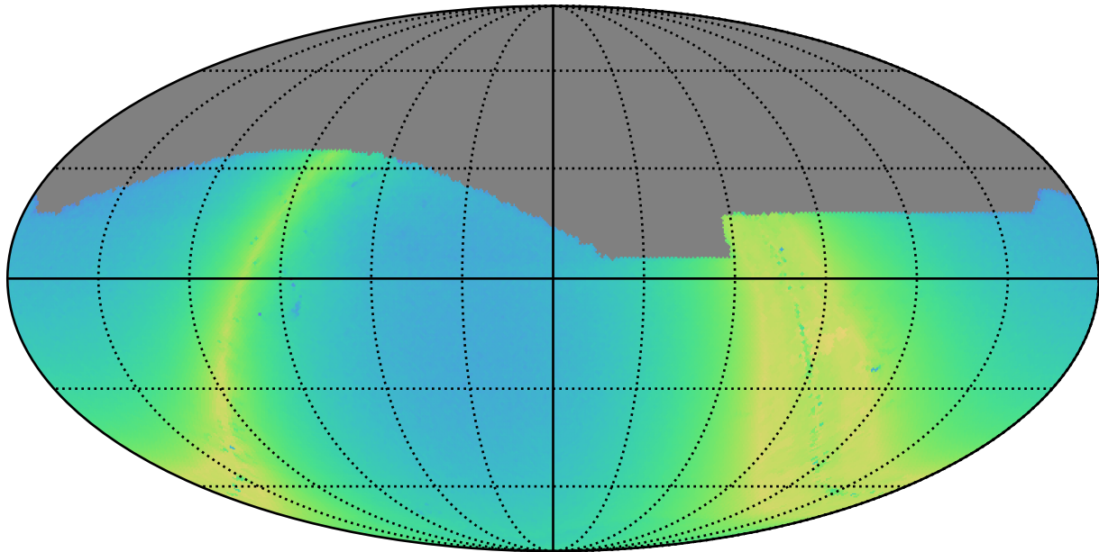
too_100_4v3.4_10yrs i: N stars to Precision 0.20
