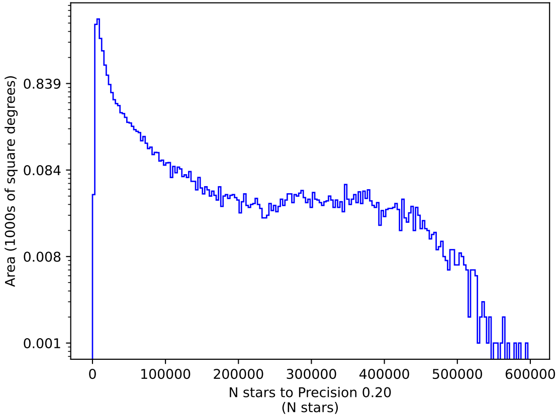
too_100_4v3.4_10yrs g: N stars to Precision 0.20
