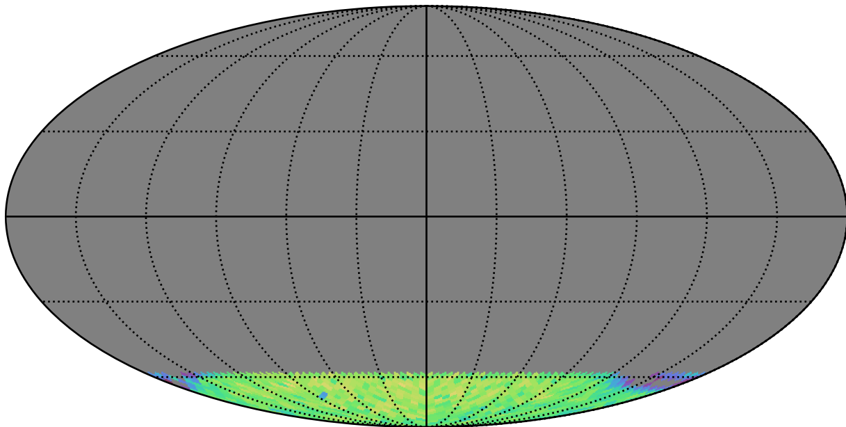
too_100_4v3.4_10yrs gi SCP: LVDwarfs
