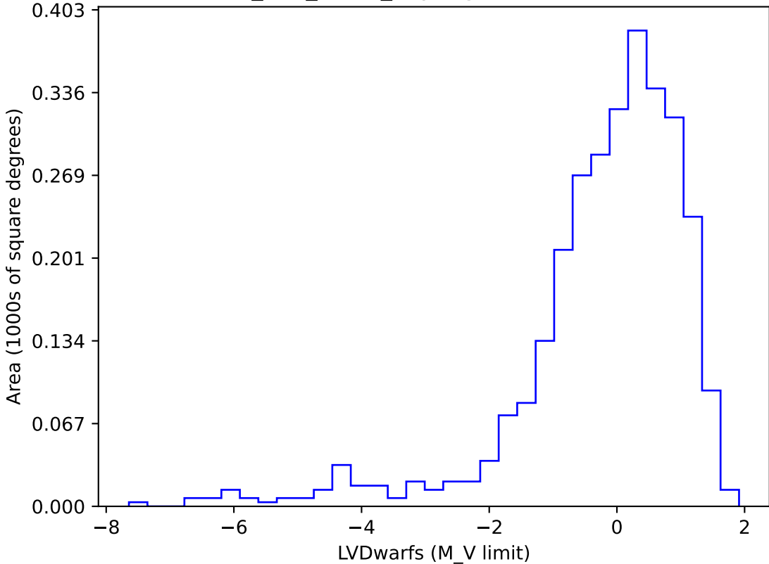
too_100_4v3.4_10yrs gi SCP: LVDwarfs
