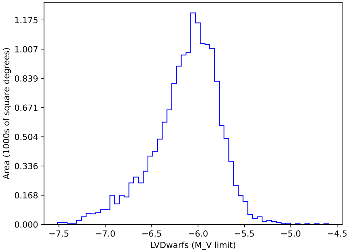
too_100_4v3.4_10yrs gi: LVDwarfs
