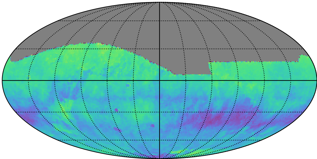
too_100_4v3.4_10yrs r: Kuiper rotSkyPos
