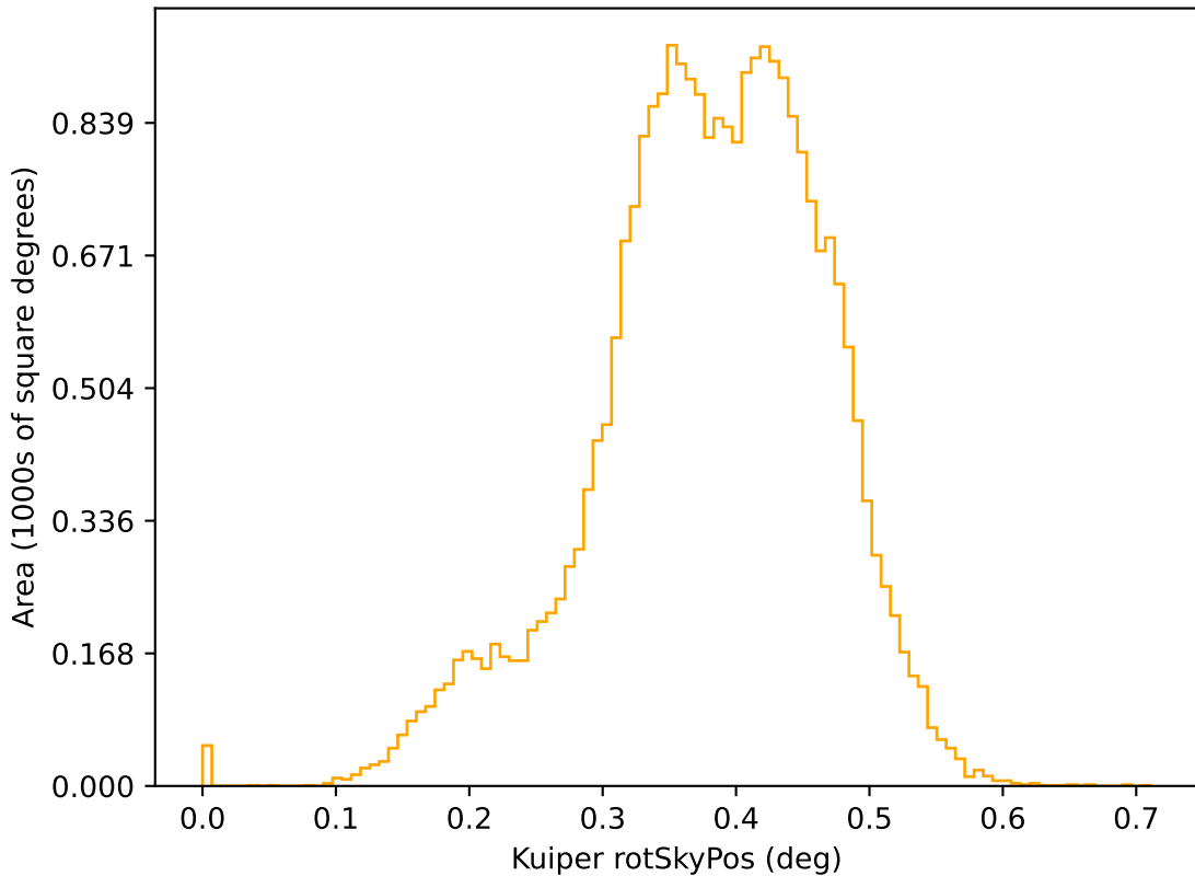
too_100_4v3.4_10yrs r: Kuiper rotSkyPos
