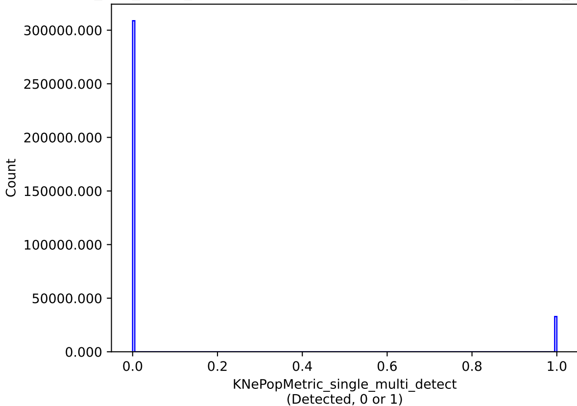
too_100_4v3.4_10yrs single model: KNePopMetric_single_multi_detect
