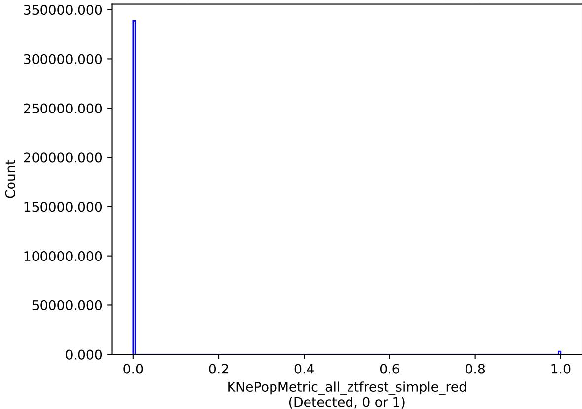
too_100_4v3.4_10yrs all models: KNePopMetric_all_ztfrest_simple_red
