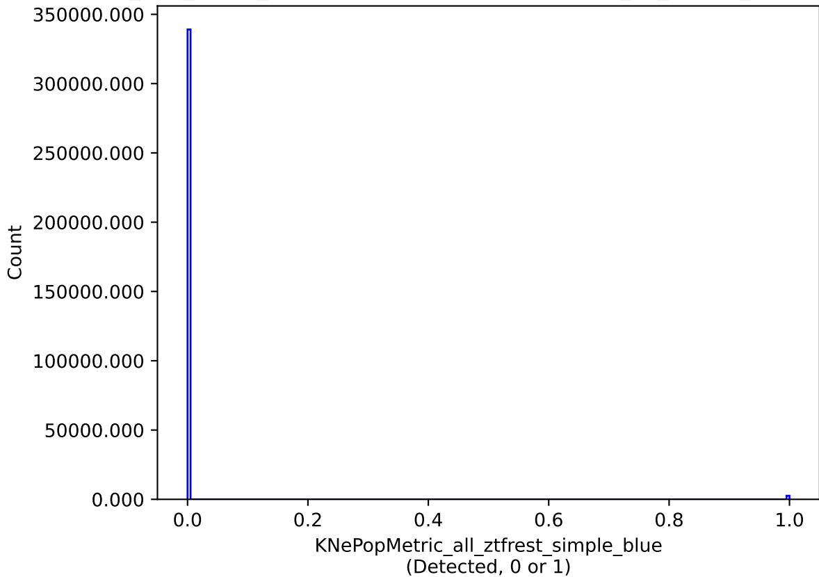
too_100_4v3.4_10yrs all models: KNePopMetric_all_ztfrest_simple_blue
