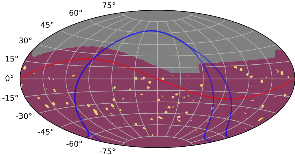
too_100_4v3.4_10yrs all models: KNePopMetric_all_ztfrest_simple
