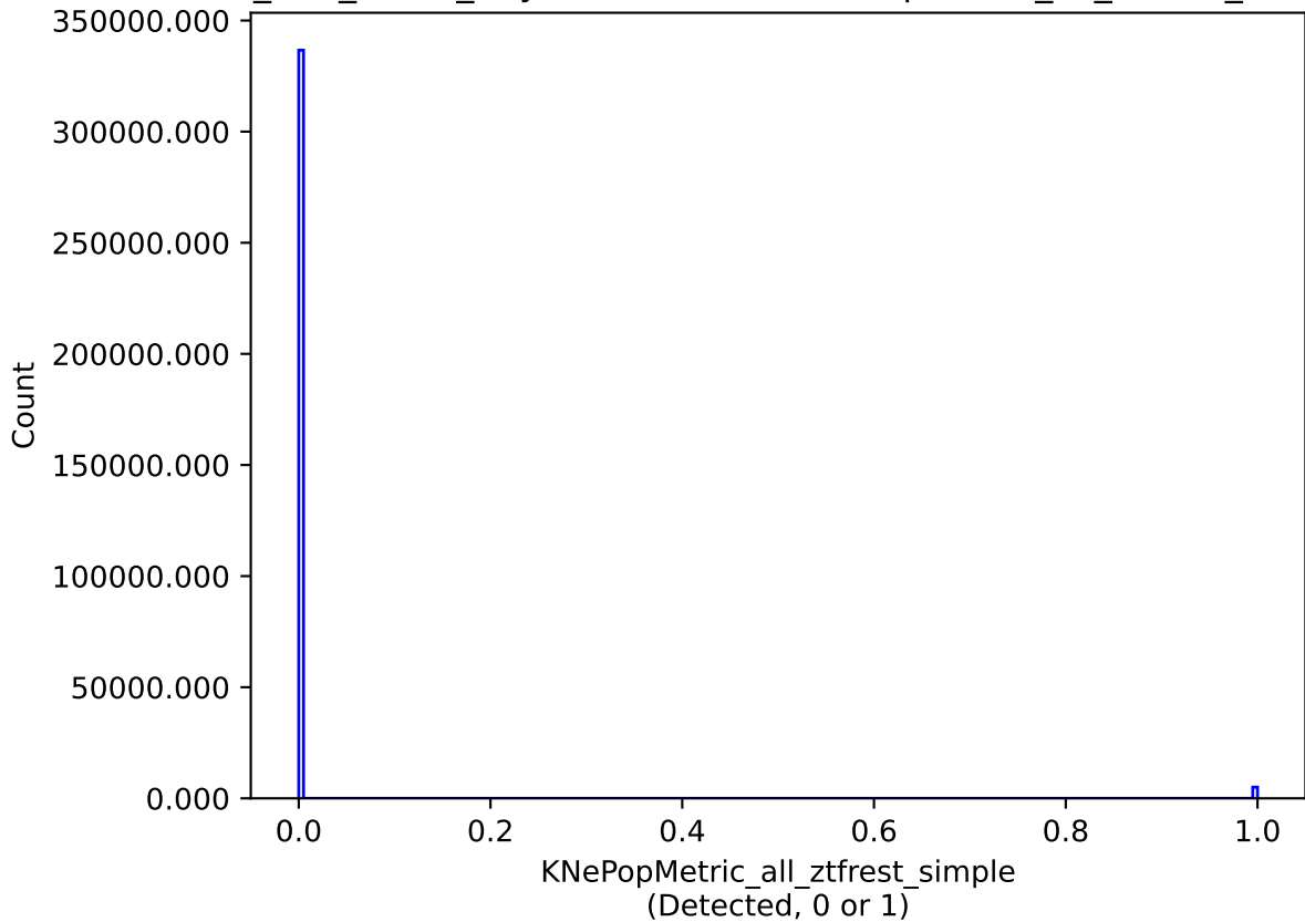
too_100_4v3.4_10yrs all models: KNePopMetric_all_ztfrest_simple
