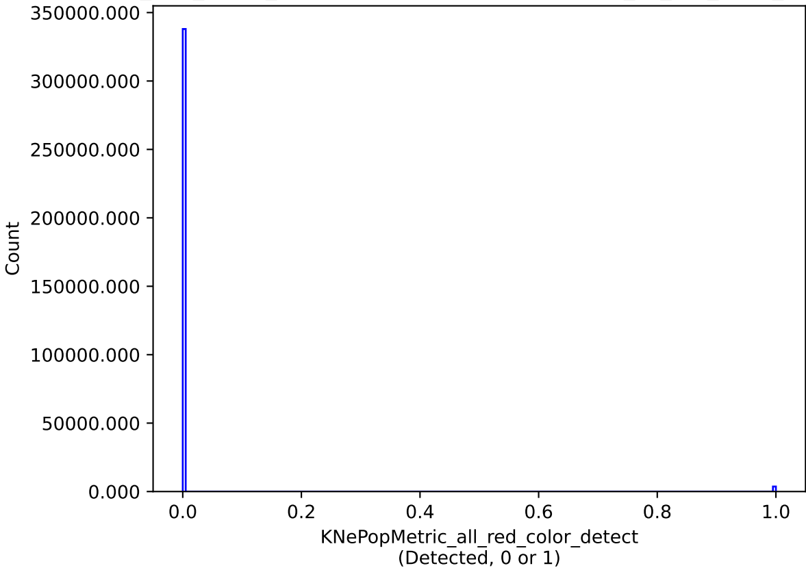
too_100_4v3.4_10yrs all models: KNePopMetric_all_red_color_detect
