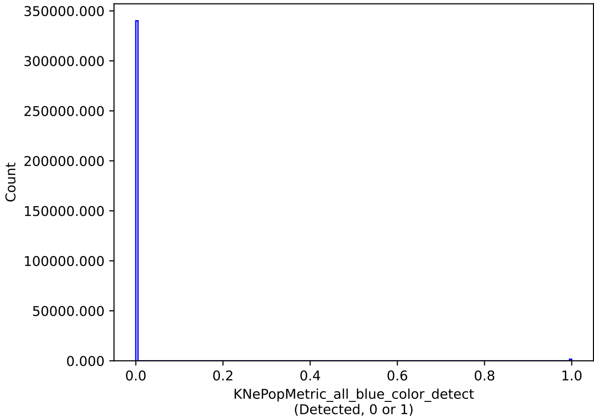
too_100_4v3.4_10yrs all models: KNePopMetric_all_blue_color_detect
