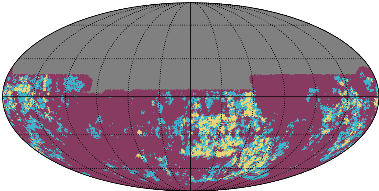
too_100_4v3.4_10yrs y band: Gaps_7hr
