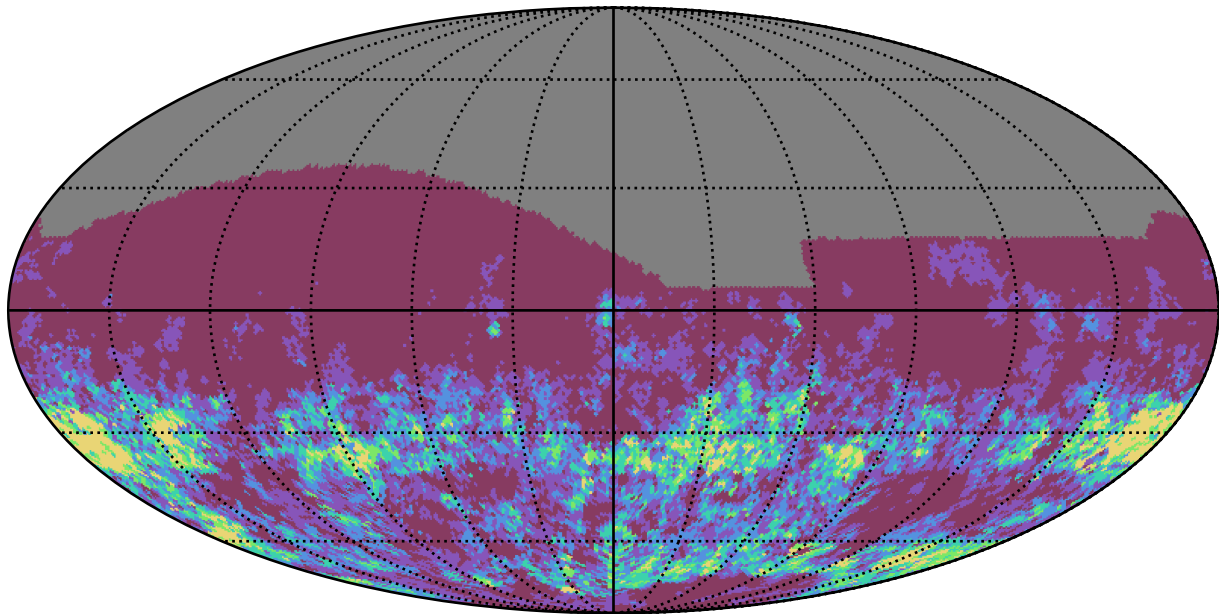
too_100_4v3.4_10yrs r band: Gaps_7hr
