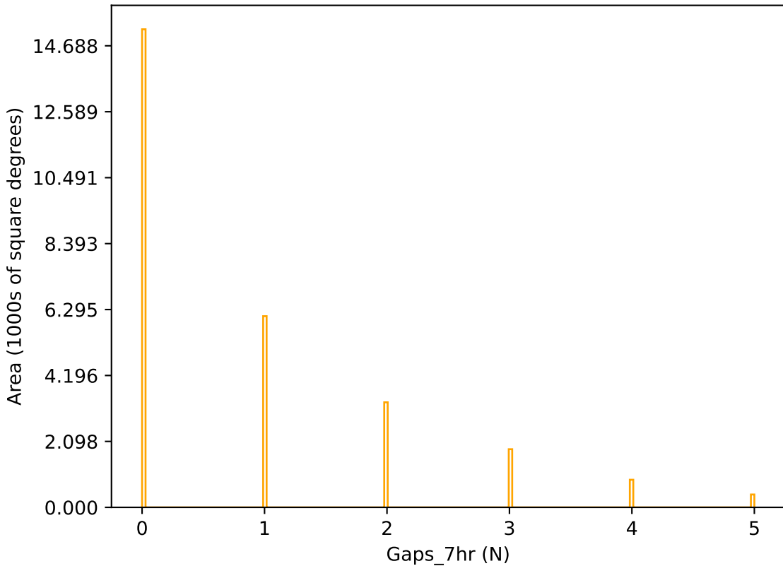
too_100_4v3.4_10yrs r band: Gaps_7hr
