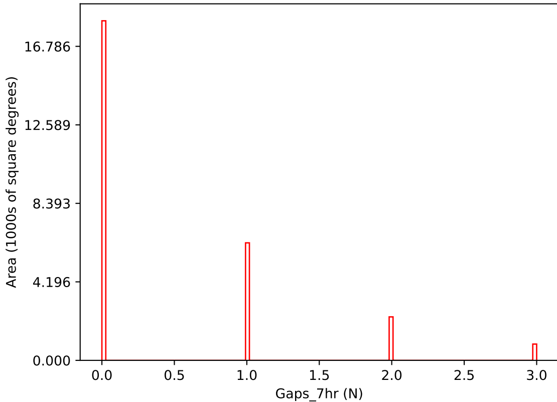
too_100_4v3.4_10yrs i band: Gaps_7hr
