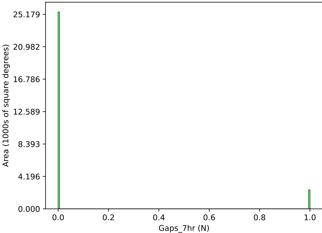
too_100_4v3.4_10yrs g band: Gaps_7hr
