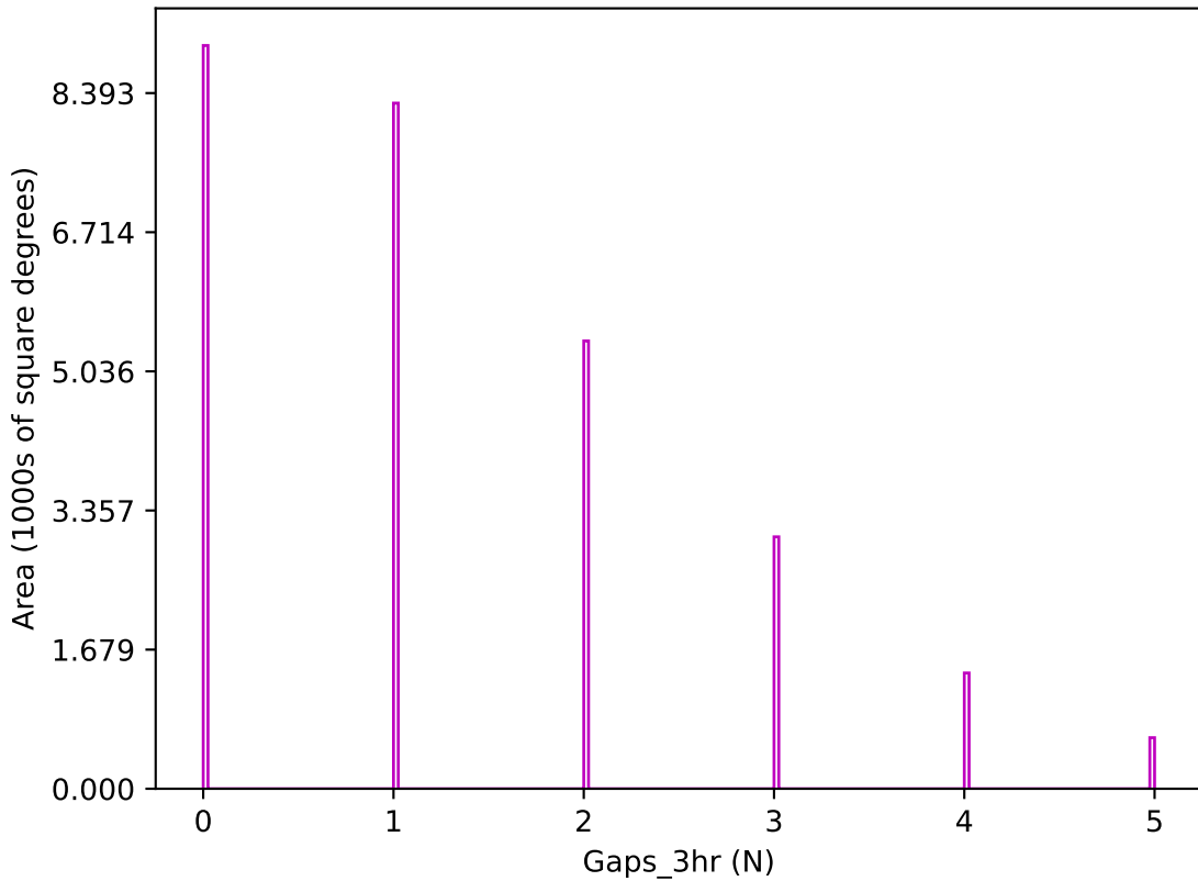
too_100_4v3.4_10yrs z band: Gaps_3hr
