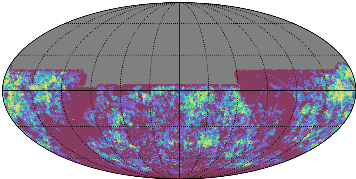
too_100_4v3.4_10yrs y band: Gaps_3hr
