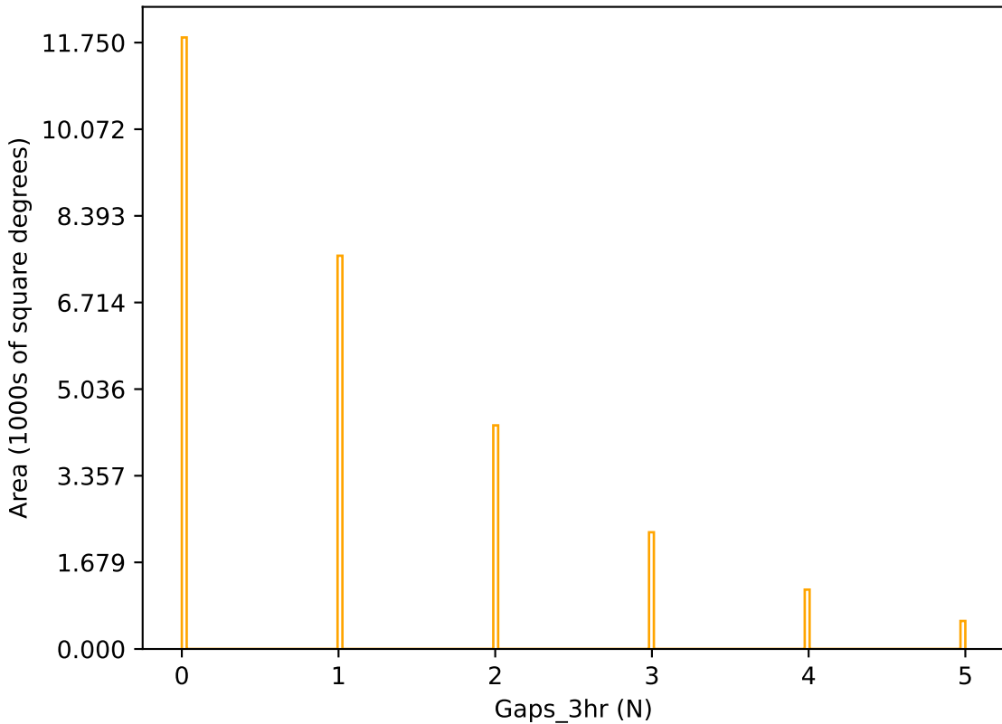
too_100_4v3.4_10yrs r band: Gaps_3hr
