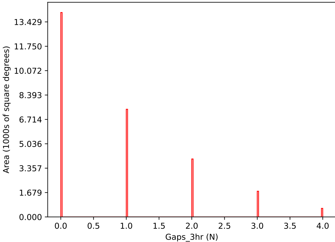
too_100_4v3.4_10yrs i band: Gaps_3hr
