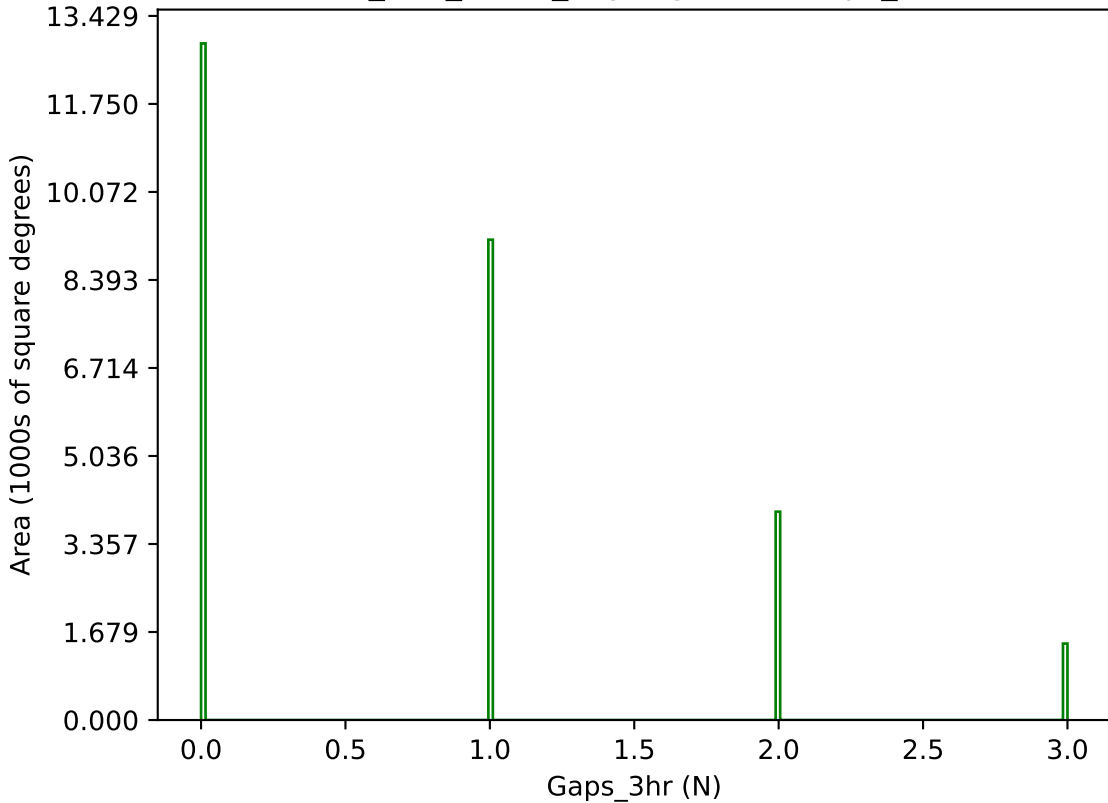
too_100_4v3.4_10yrs g band: Gaps_3hr
