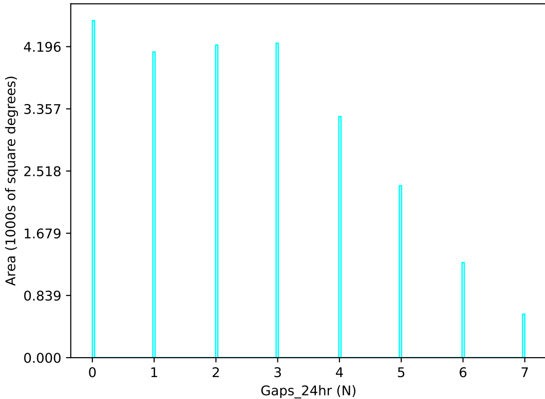
too_100_4v3.4_10yrs u band: Gaps_24hr
