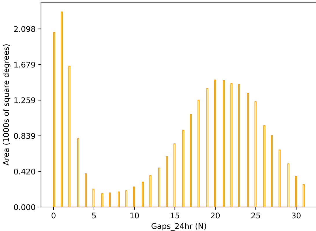
too_100_4v3.4_10yrs r band: Gaps_24hr
