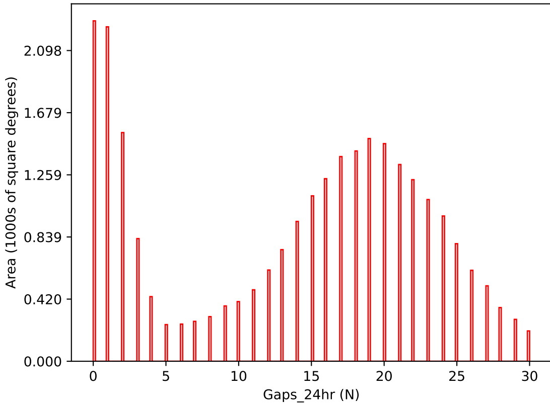
too_100_4v3.4_10yrs i band: Gaps_24hr
