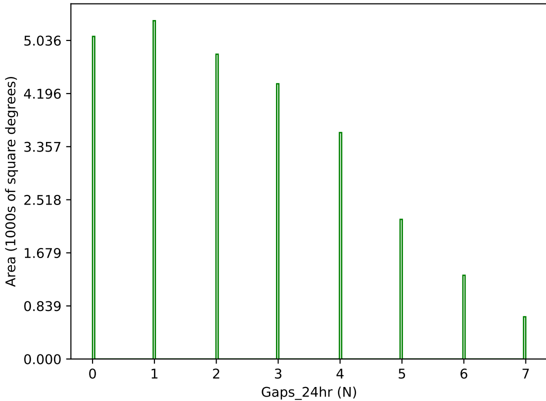
too_100_4v3.4_10yrs g band: Gaps_24hr
