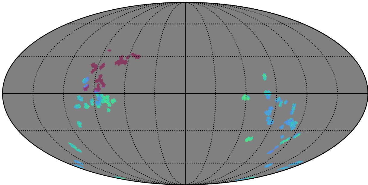
too_100_4v3.4_10yrs : GalplaneTimePerFilter_zucker_sfr_map_y
