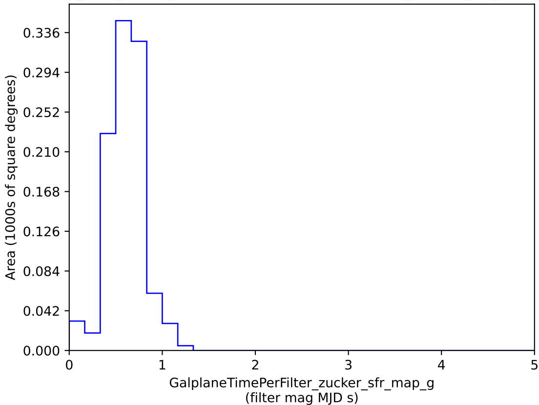
too_100_4v3.4_10yrs : GalplaneTimePerFilter_zucker_sfr_map_g
