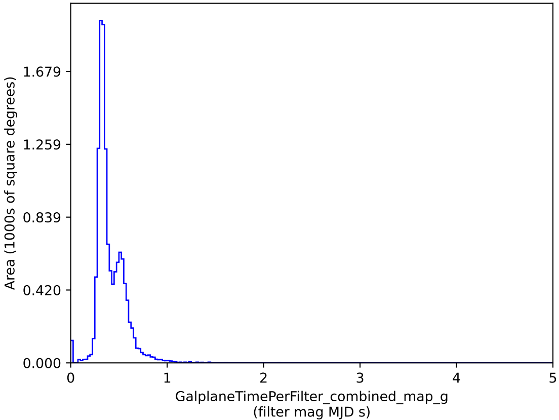
too_100_4v3.4_10yrs : GalplaneTimePerFilter_combined_map_g
